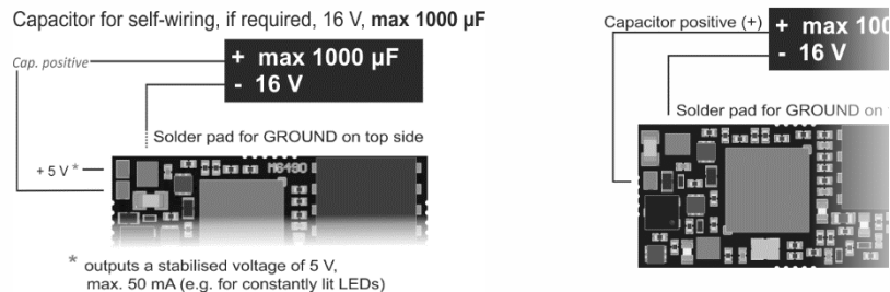
...or with ELKO on the MS490, ...R, ...F, ...N Bottom side
