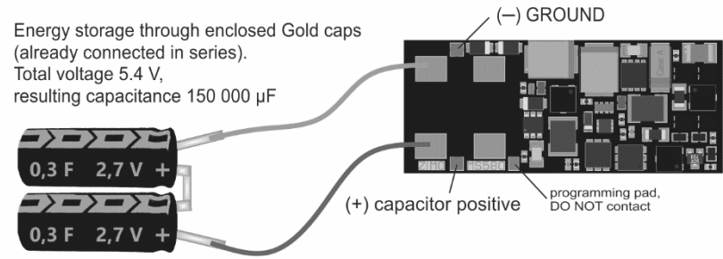
MS580N18G Bottom of the version G
